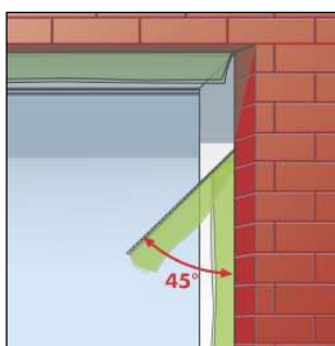
Fig. 3 Pull the film at an angle of 45°
