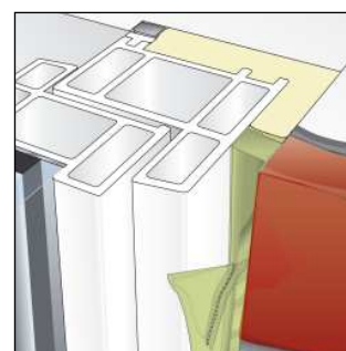
Fig. 4 TP601 Compriband e located to perimeter of window (check reveal shown)
